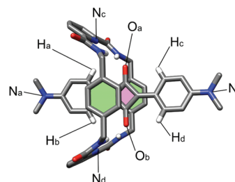
FIGURE 3. Atom labels for squaraine rotaxanes.
