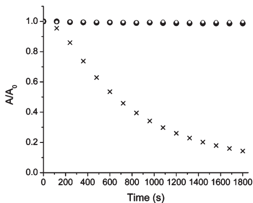
FIGURE 9. Change in absorption upon addition of 2-mercaptoethanol (50 mM) to 4 (●), 5 (○), and 1a (x) in \text{CHCl}_3 ( 10 \mu\text{M} ) at 25 \text{ }^\circ\text{C} .
