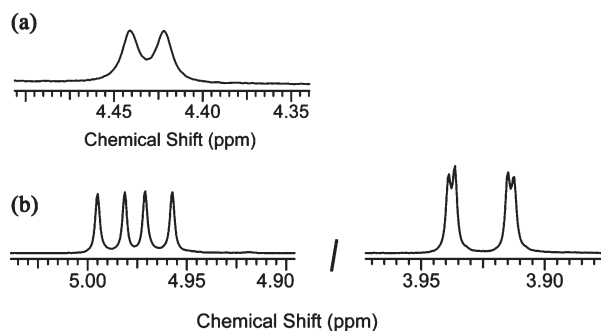
FIGURE 4. Partial ^1\text{H} NMR spectra at 22 °C in \text{CDCl}_3 showing the macrocycle methylene signals for squaraine rotaxanes: (a) 2d with J = 5.8 Hz in a 300 MHz spectrum; (b) 5 with J_1 = 8.2 Hz, J_2 = 14.4 Hz (left) and J_1 = 1.5 Hz, J_2 = 14.4 Hz (right) in a 600 MHz spectrum.
