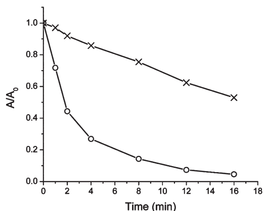
FIGURE 8. Change in absorption of 4 (O) and 5 (x) in \text{CHCl}_3 ( 10 \mu\text{M} ) upon exposure to an unfiltered xenon arc lamp (150 W) at 25 \text{ }^\circ\text{C} .
